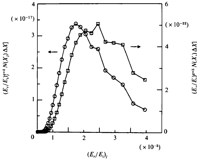
FIGURE 12. Values of (E_r/E_t)_i raised to the fourth and fifth powers, weighted by their number of occurrences N(X_j)\Delta X . \circ , q = 4 ; \square , q = 5 , both for a typical box size r = 64\eta .
