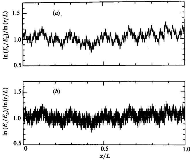
FIGURE 5. Local values of \alpha = \ln(E_r/E_p)/\ln(r/L) for (a) r/L = 2^{-9} after 9 steps, and (b) for r/L = 2^{-13} after 13 steps.
