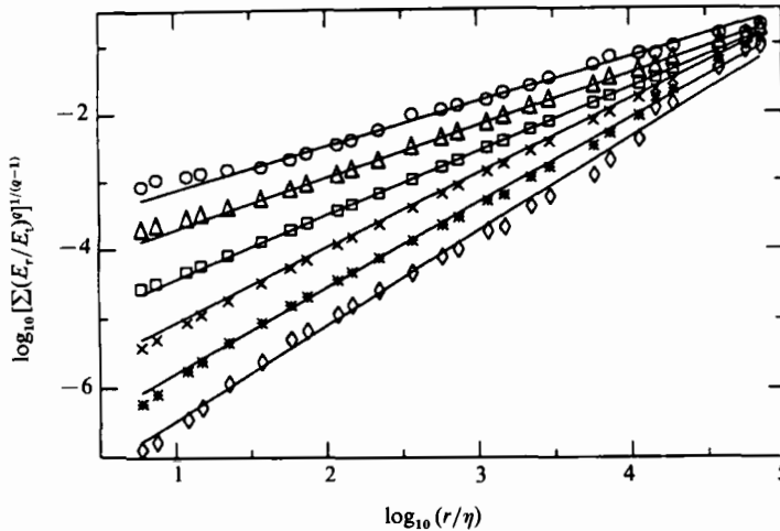
FIGURE 22. Log-log plots of [\sum (E_r/E_c)^q]^{1/(q-1)} as a function of r/\eta for the flow in the atmospheric surface layer. \circ , q = 4 ; \triangle , q = 2 ; \square , q = 0.6 ; \times , q = -0.6 ; * , q = -2 ; \diamond , q = -4 . Solid lines are linear least-square fits in the range r/\eta = 10 to 30000.
