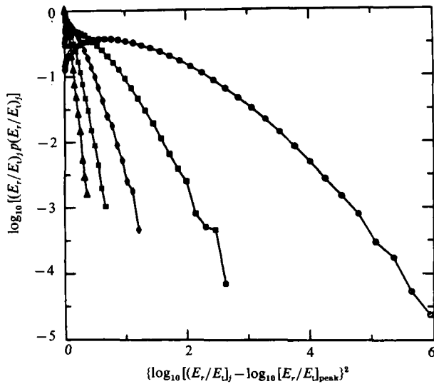
FIGURE 26. High-intensity tails of the probability density of E_r/E_t , plotted such that a linear behaviour at the tails indicates a lognormal distribution. Different symbols correspond to different box sizes as in figure 11.
